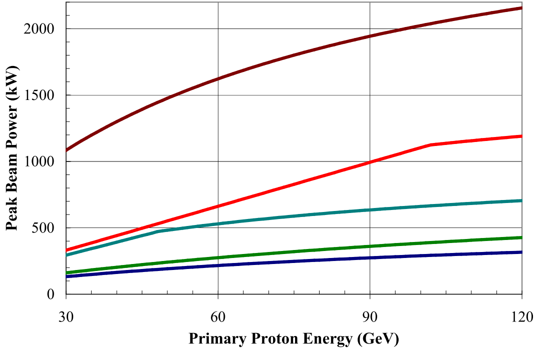
Figure 14: Preliminary estimates of increasing proton beam power in kWatt as a function of proton energy at Fermilab.
