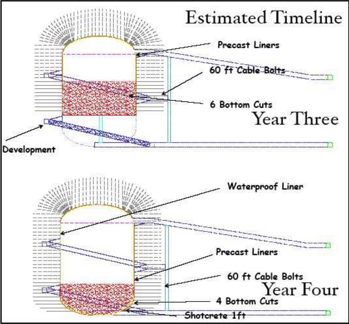
Figure 13: Details of the construction of a single cavern in year 3 and 4.
