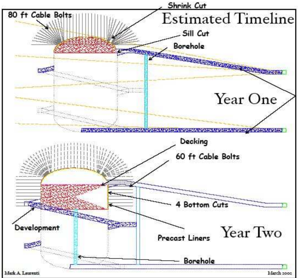
Figure 12: Details of the construction of a single cavern.
