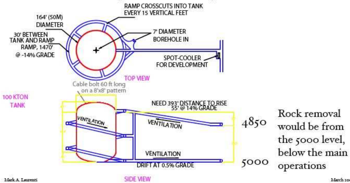
Figure 11: Details of the construction of a single cavern.
