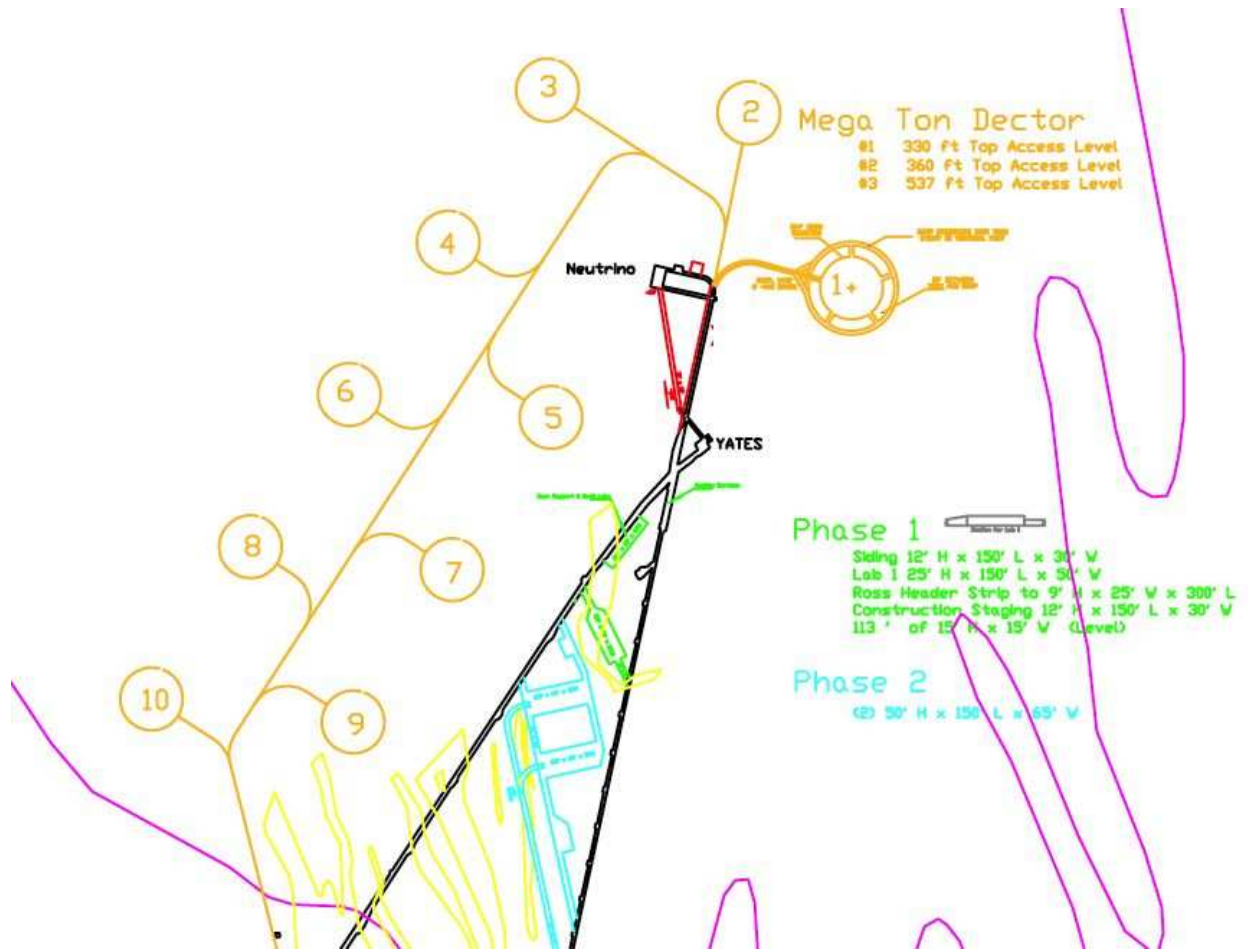
Figure 10: Possible linear layout of 10 caverns at Homestake. This layout is developed for the 4850 ft level. The location of the Davis Chlorine cavern is indicated by the word “neutrino”.
