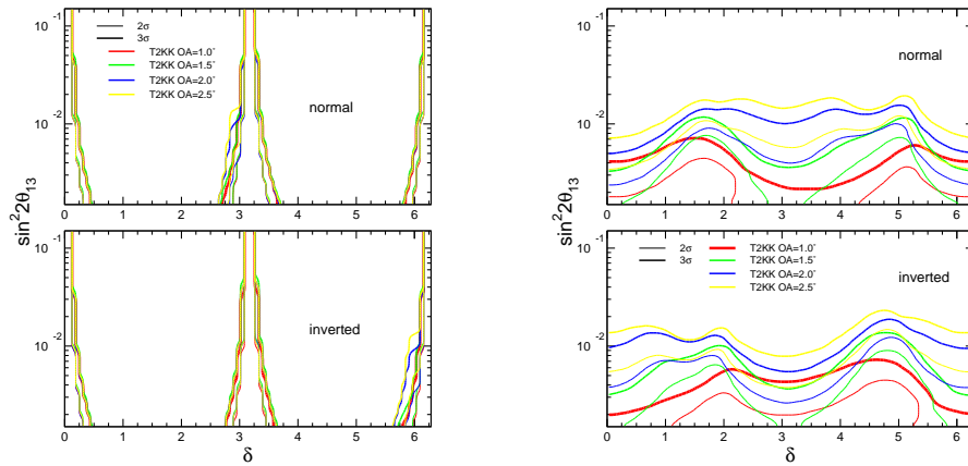
Fig. 7 Sensitivity to CP violation (left) and mass hierarchy (right) for different values of the off-axis angle. (Other parameters: \Delta m_{(21,31)}^2 = 7.3 \times 10^{-5}, 2.5 \times 10^{-3} eV^2 and the other mixing angles: \sin^2 2\theta_{(12,23)} = 0.86, 1.0 . We assumed the earth density to be constant and to be equal to 2.8 g/cm^3 )
