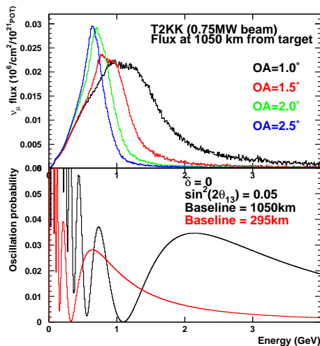
Fig. 1 Neutrino flux as a function of energy for several off-axis angle, and a 0.75MW beam at 1050km from the target. For comparison, the \nu_\mu \rightarrow \nu_e probability, for the two baseline considered in T2KK (295km and 1050km), for \Delta m_{(21,31)}^2 = 7.3 \times 10^{-5}, 2.5 \times 10^{-3} eV^2 and the other mixing angles at \sin^2 2\theta_{(12,23)} = 0.86, 1.0 . We assumed the earth density to be constant and to be equal to 2.8 g/cm^3
