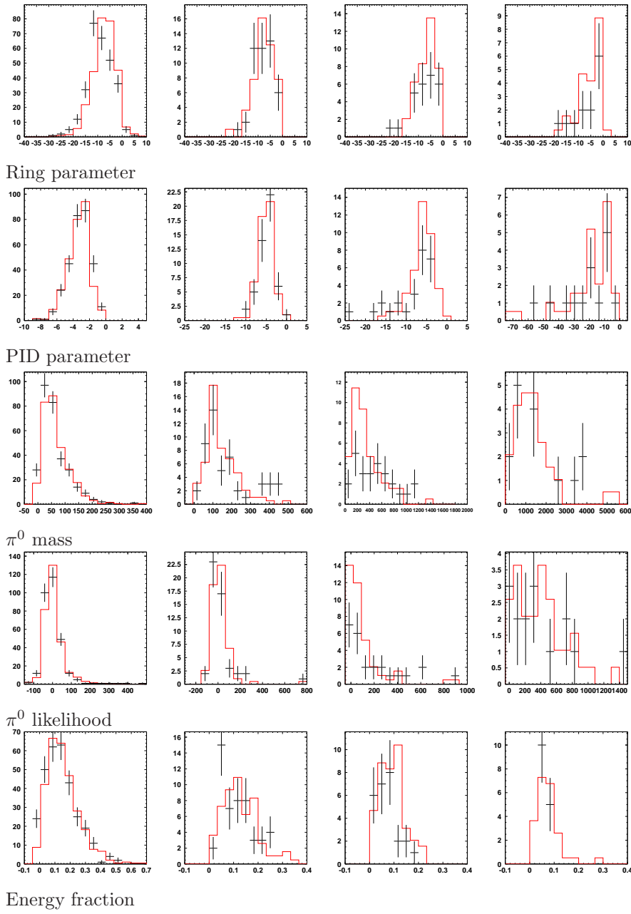
Fig. 3 Comparison of data and Monte Carlo for five likelihood variables. Black = 1489 days of SK atmospheric data, Red = 9 years of SK atmospheric Monte Carlo normalized to the data livetime.
