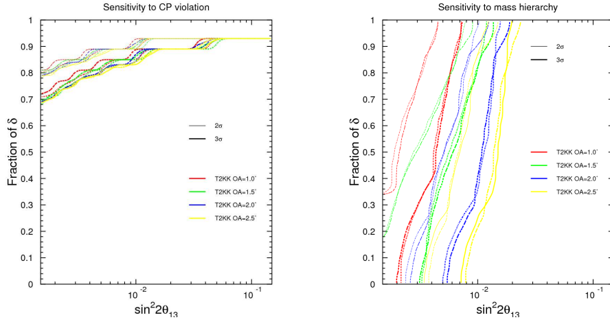
Fig. 6 Sensitivity to CP violation (left) and mass hierarchy (right) for different values of the off-axis angle. (Other parameters: \Delta m_{(21,31)}^2 = 7.3 \times 10^{-5}, 2.5 \times 10^{-3} eV^2 and the other mixing angles: \sin^2 2\theta_{(12,23)} = 0.86, 1.0 . We assumed the earth density to be constant and to be equal to 2.8 g/cm^3 )
