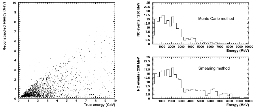
Fig. 8 left: Smearing matrix for NC events, Right: Comparison of methods to compute NC background: Top plot is the MC method, bottom plot is the smearing method. The plots are normalized for 30 \times 10^{20} POT and a 300kTon detector.
