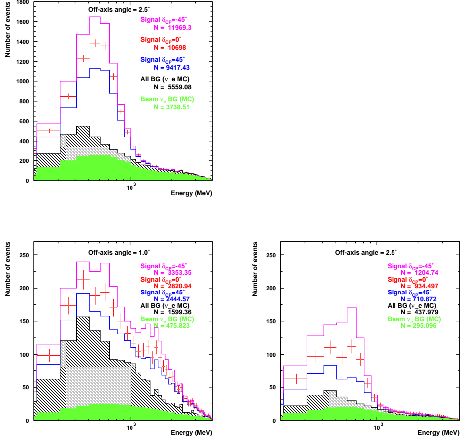
Fig. 5 Spectrum at Kamioka (top), Korea 1.0° off-axis (bottom left) and Korea 2.5° off-axis (bottom right) for \sin^2(2\theta_{13}) = 0.04 . The remaining oscillation parameters are: \Delta m_{(21,31)}^2 = 7.3 \times 10^{-5}, 2.5 \times 10^{-3} eV^2 and the other mixing angles: \sin^2 2\theta_{(12,23)} = 0.86, 1.0 . We assumed the earth density to be constant and to be equal to 2.8 g/cm^3
