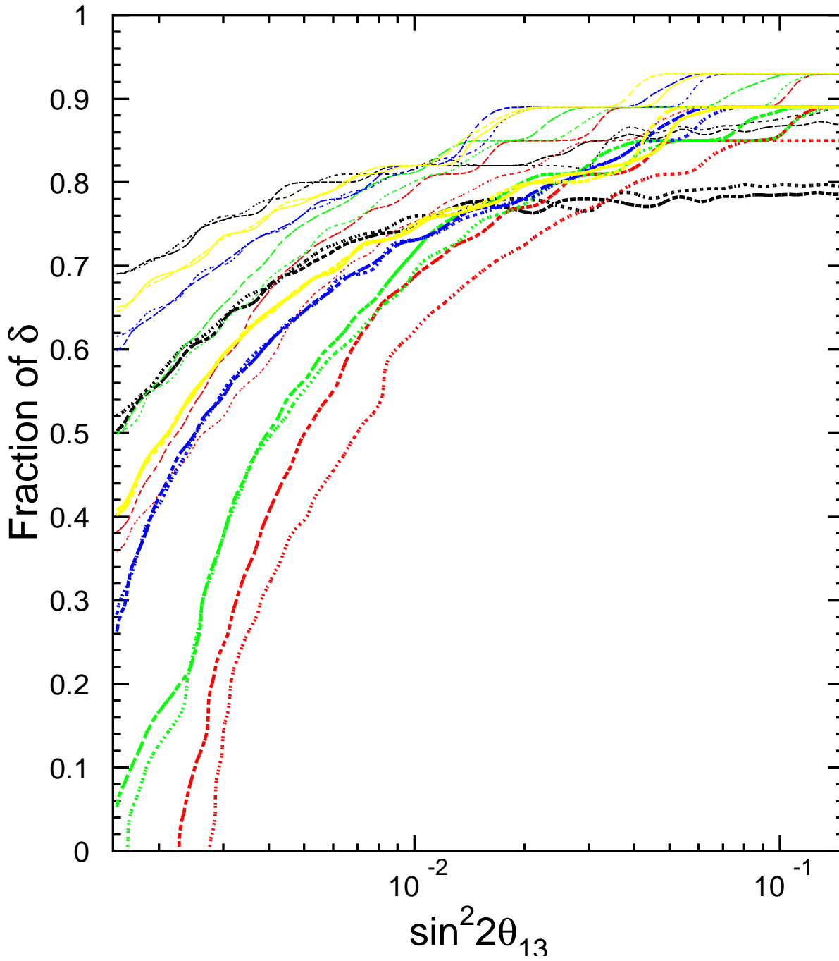
Sensitivity to CP violation
