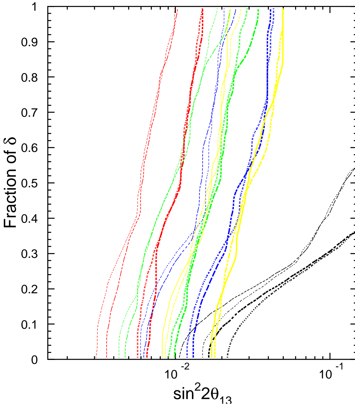
Sensitivity to mass hierarchy
