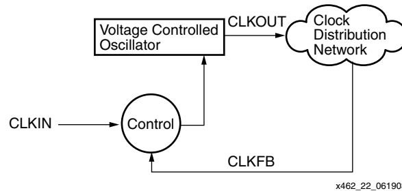
Figure 3-21: Phase-Locked Loop (PLL) Block Diagram
