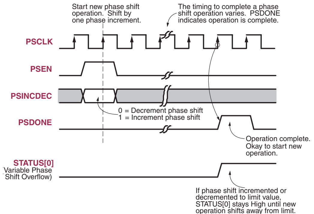
Figure 3-34: Dynamic Fine Phase Shift Control Interface
