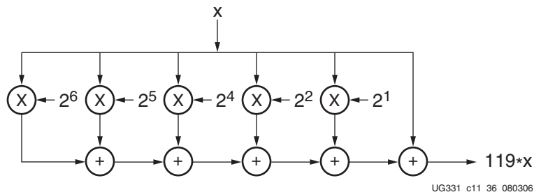
Figure 9-36: Binary Multiplication by 119 Uses 5 Multipliers and 5 Adders
