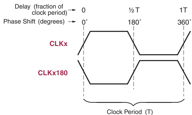
Figure 3-26: Half-Period Phase Shift Outputs
