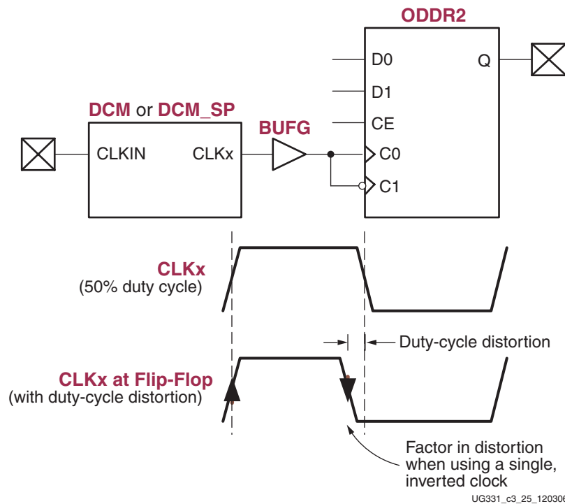
Figure 3-27: Dual-Data Rate (DDR) Output Using Both Edges of a Single Clock Induces Duty-Cycle Distortion
