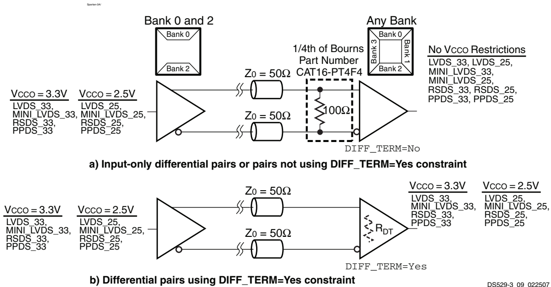
Figure 10-31: External Input Termination Resistors for Spartan-3A/3AN/3A DSP LVDS, RSDS, MINI_LVDS, and PPDS I/O Standards
