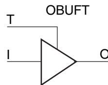
Figure 10-6: 3-State Output Buffer (OBUFT) Symbol
