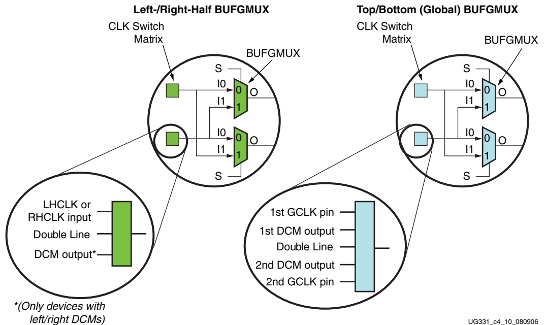
Figure 2-10: Spartan-3E/3A/3AN/3A DSP Clock Switch Matrix for BUFGMUX Pair Connectivity
