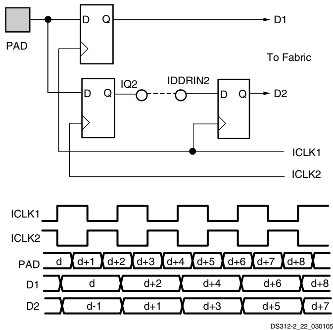
Figure 10-16: Input DDR Using Cascade Feature
