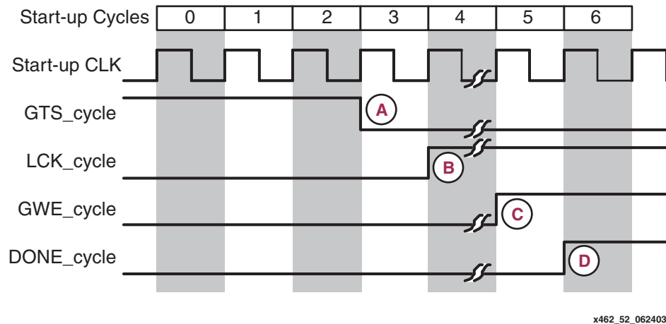
Figure 3-52: Start-up Logic Interaction with DCM LOCKED Output
