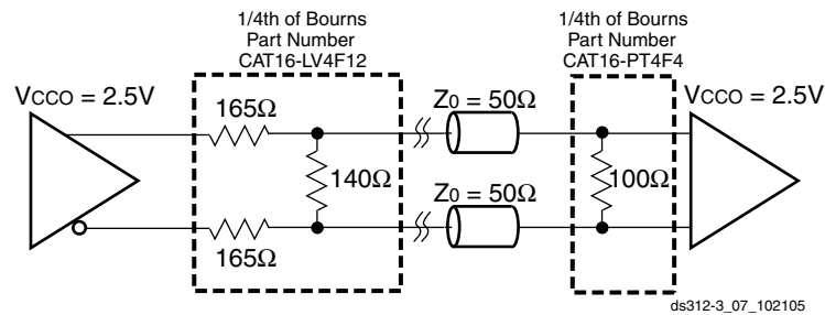
Figure 10-33: External Termination Resistors for BLVDS I/Os
