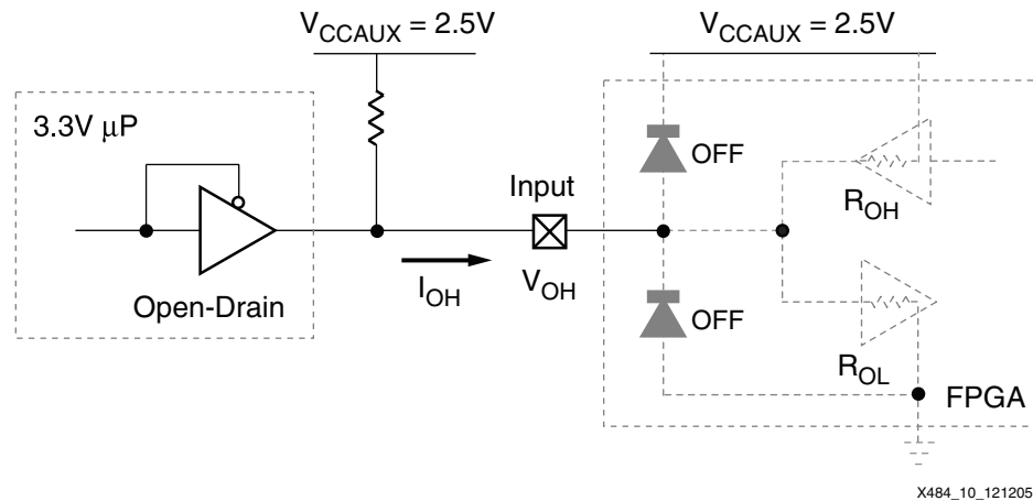
Figure 10-38: A 3.3V Open-Drain Output Connected to an FPGA's Dedicated Input
