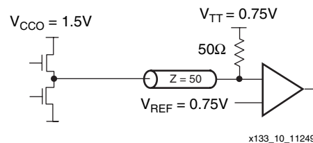
Figure 10-23: Terminated HSTL Class I
