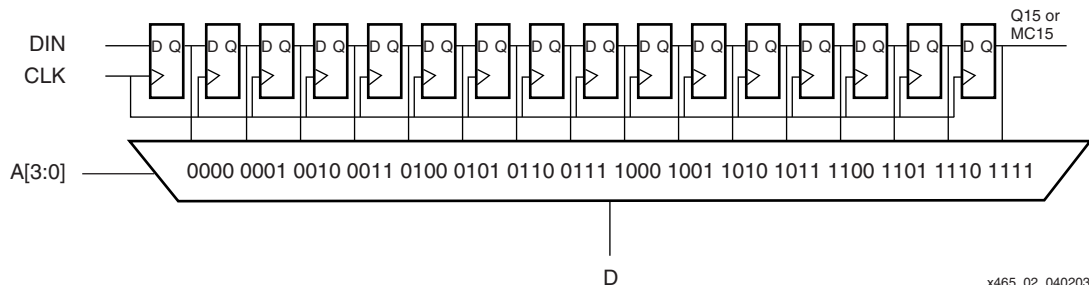
Figure 7-2: LUT Configured as an Addressable Shift Register
