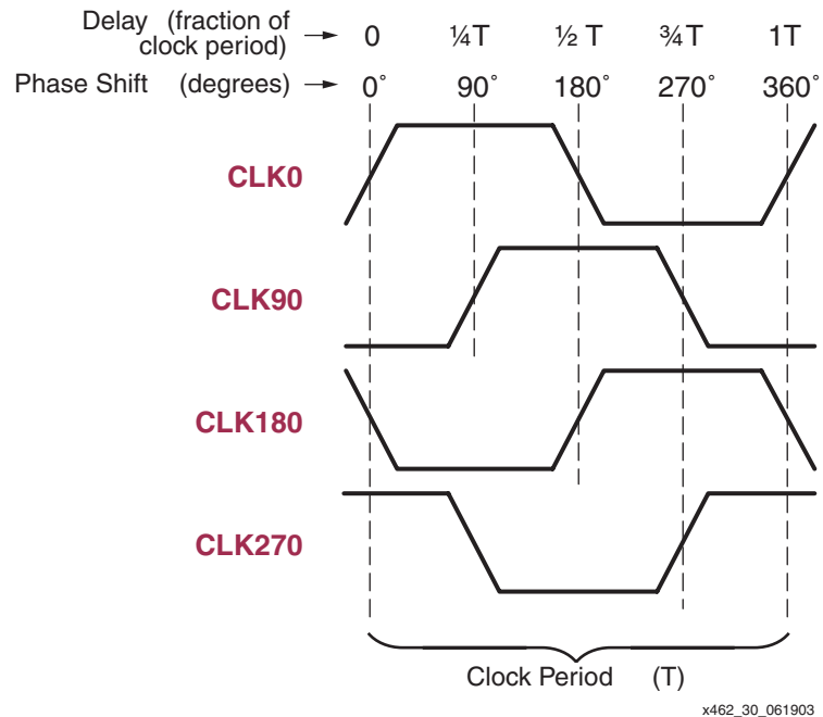
Figure 3-29: Quadrant Phase Shift Outputs Shift CLKIN, Each by a Quarter Period (Shown with Duty-Cycle Correction Enabled)
