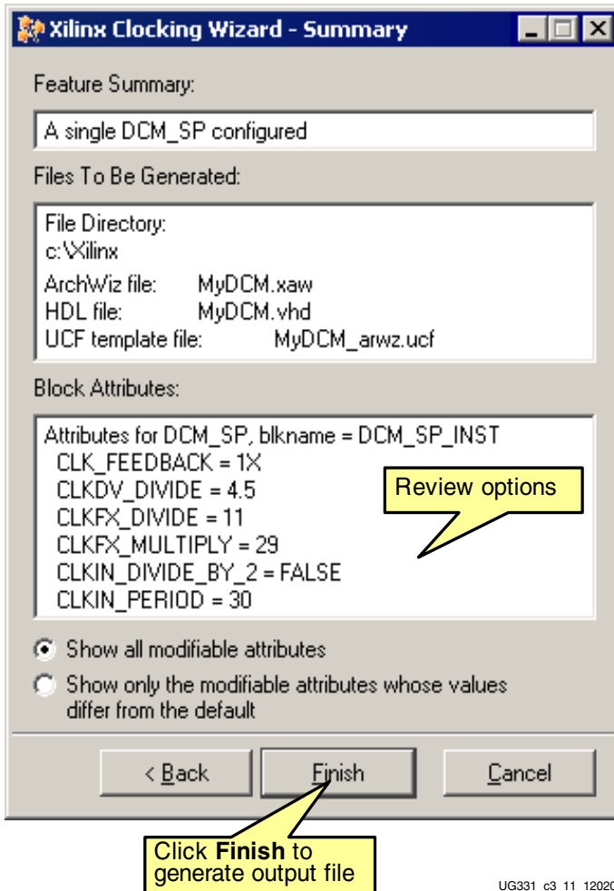
Figure 3-13: Review Settings, Then Click Finish
