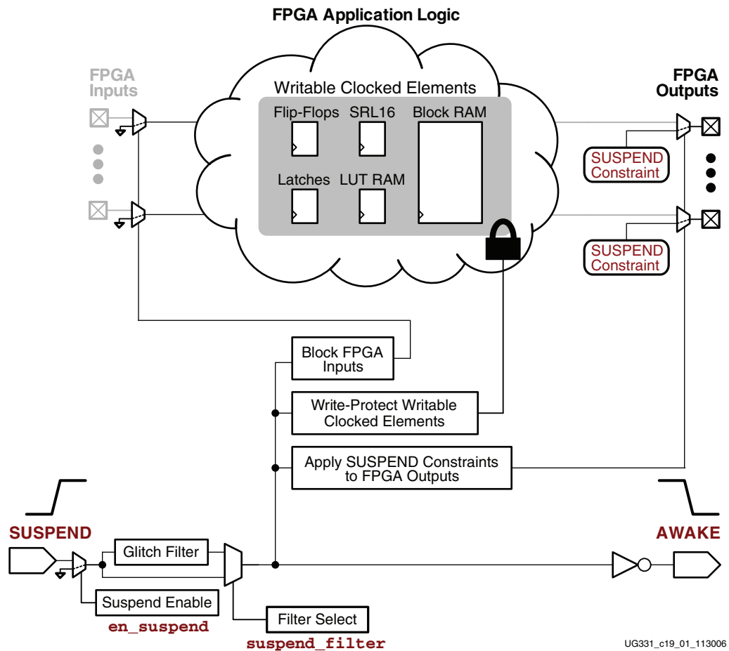
Figure 19-2: Entering Spartan-3A/3AN/3A DSP Suspend Mode
