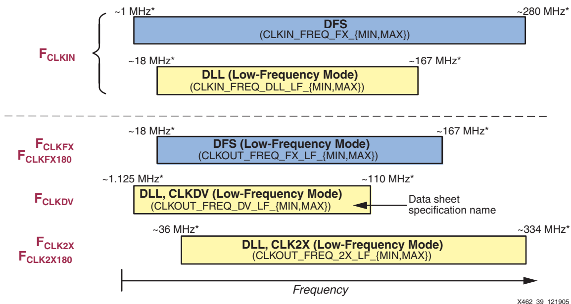
Figure 3-39: Input and Output Clock Frequency Restrictions (Spartan-3 FPGA Family, Low-Frequency Mode Example)
