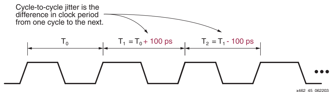
Figure 3-45: Cycle-to-Cycle Jitter Example
