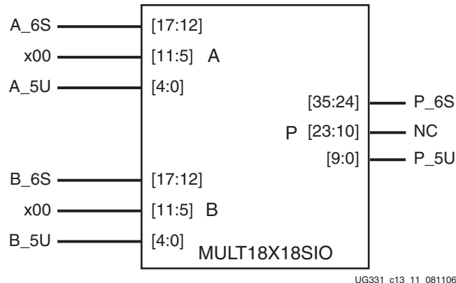
Figure 11-8: Two Multipliers in One Primitive
