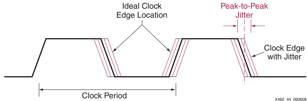
Figure 3-44: Jitter in Clock Signals
