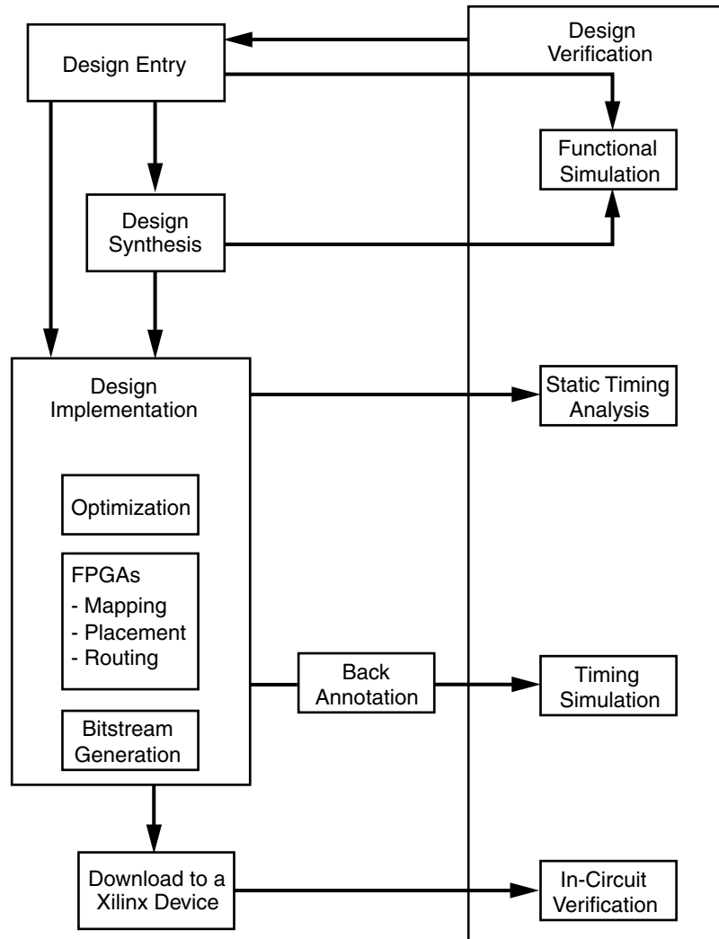
Figure 13-1: Design Flow
