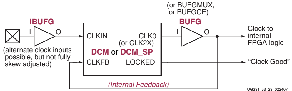
Figure 3-18: Eliminating Skew on Internal Clock Signals
