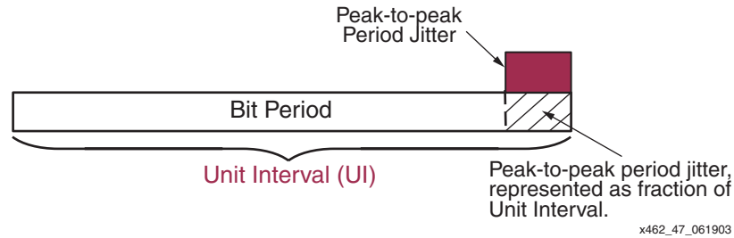
Figure 3-47: Period Jitter Specified as a Fraction of a Unit Interval
