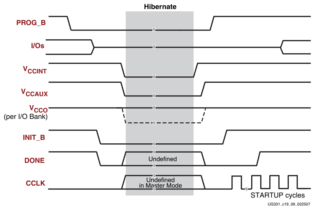
Figure 19-10: Hibernate Mode Waveform
