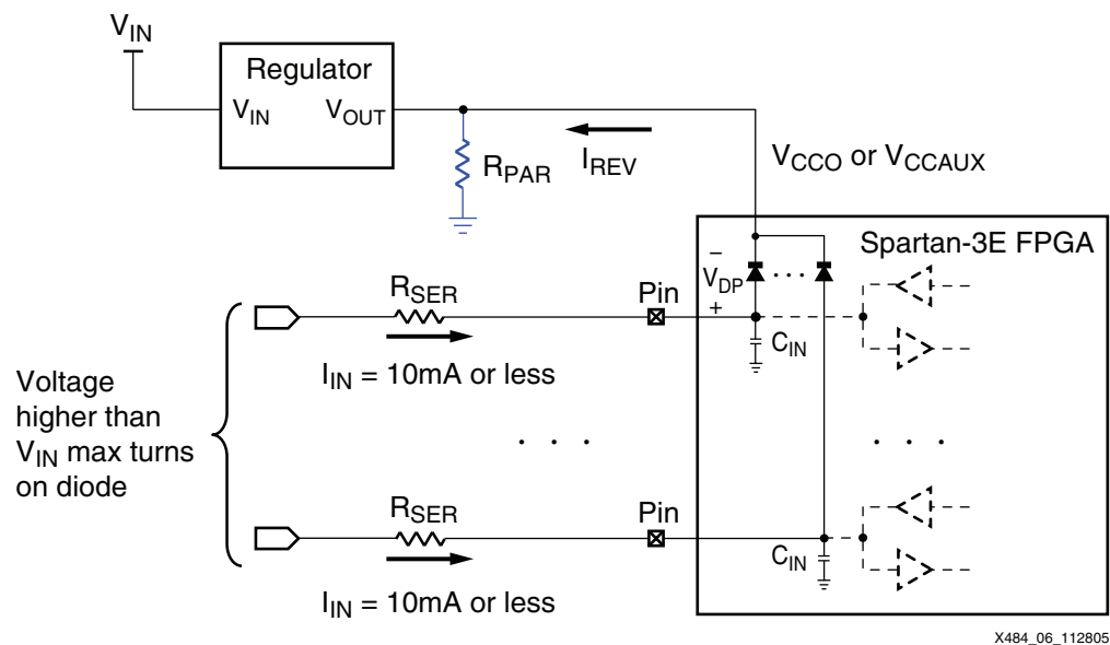
Figure 10-37: Reverse Current Solution for Regulator
