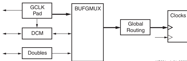
Figure 2-1: Overall View of Clock Connections
