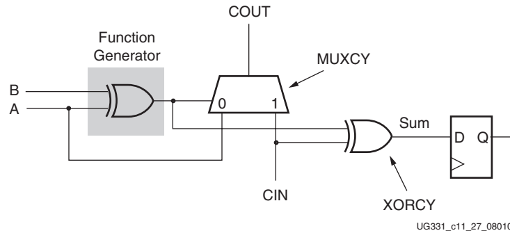
Figure 9-27: Basic Adder Cell
