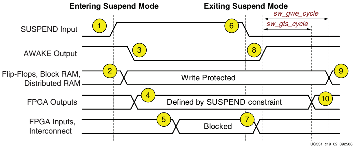
Figure 19-3: Suspend Mode Waveforms (Entering and Exiting)
