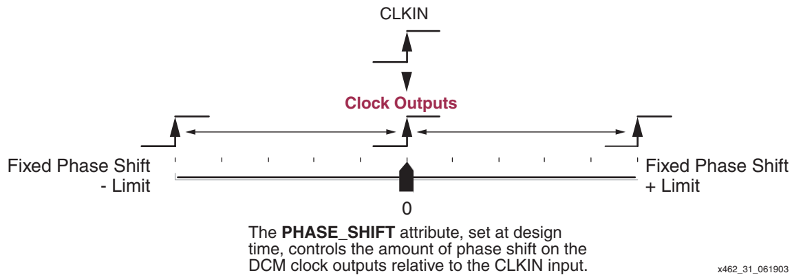
Figure 3-31: Fixed-Value Fine Phase Shift Control
