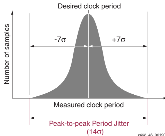
Figure 3-46: Peak-to-Peak Period Jitter Example
