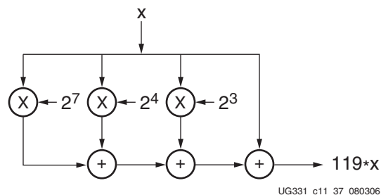
Figure 9-37: CSD Multiplication by 119 Uses 3 Multipliers and 3 Adders
