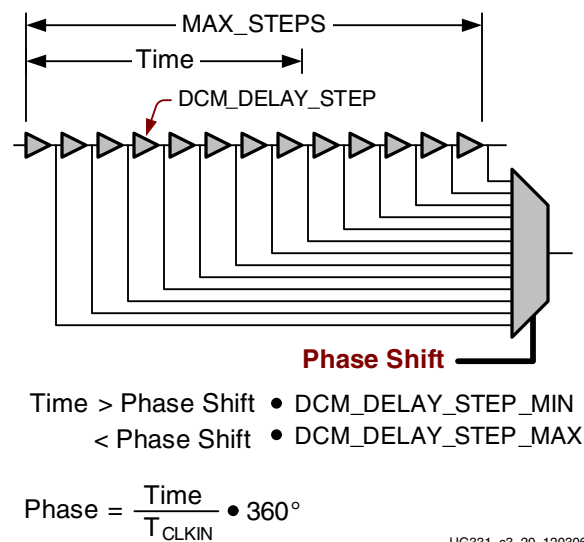
Figure 3-33: Spartan-3E and Spartan-3A/3AN/3A DSP Variable Phase Shift Logic
