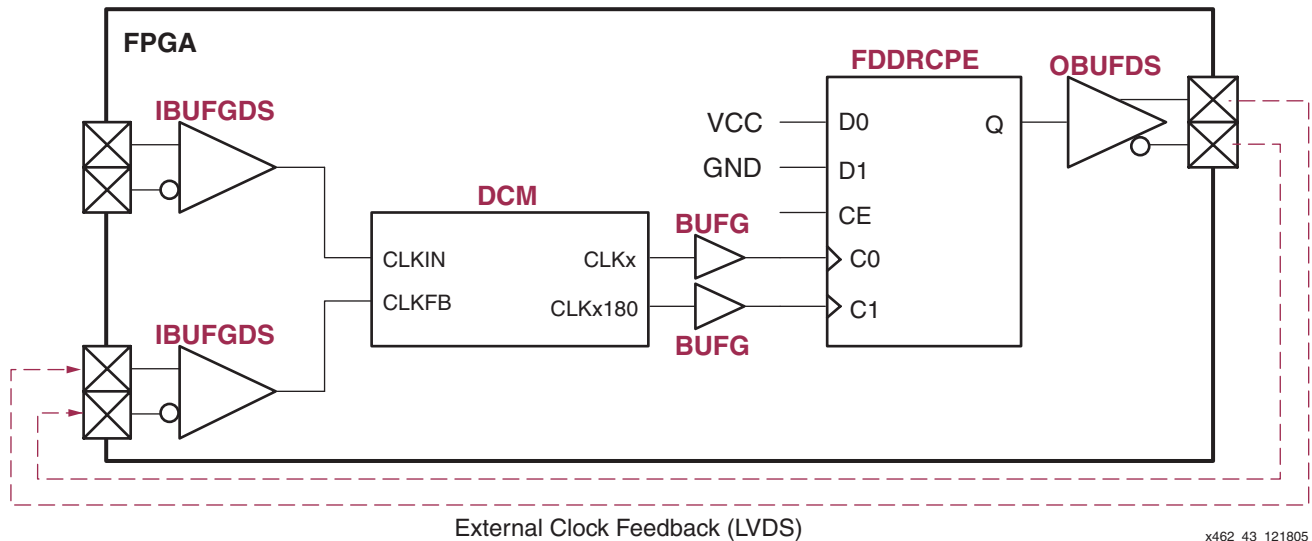
Figure 3-43: High-Frequency (250+ MHz) LVDS Clock Forwarding Circuit with 50% Duty Cycle
