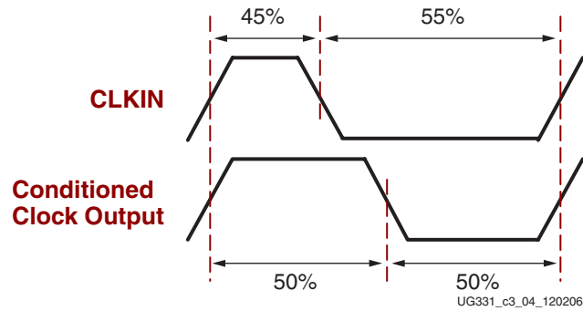
Figure 3-25: DCM Duty-Cycle Correction Feature Provides 50% Duty Cycle Outputs
