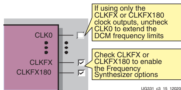
Figure 3-41: Enabling Frequency Synthesizer in Clocking Wizard
