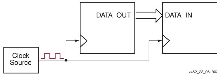
Figure 3-22: System-Synchronous Applications are Clocked by a Single, System-Wide Clock Source
