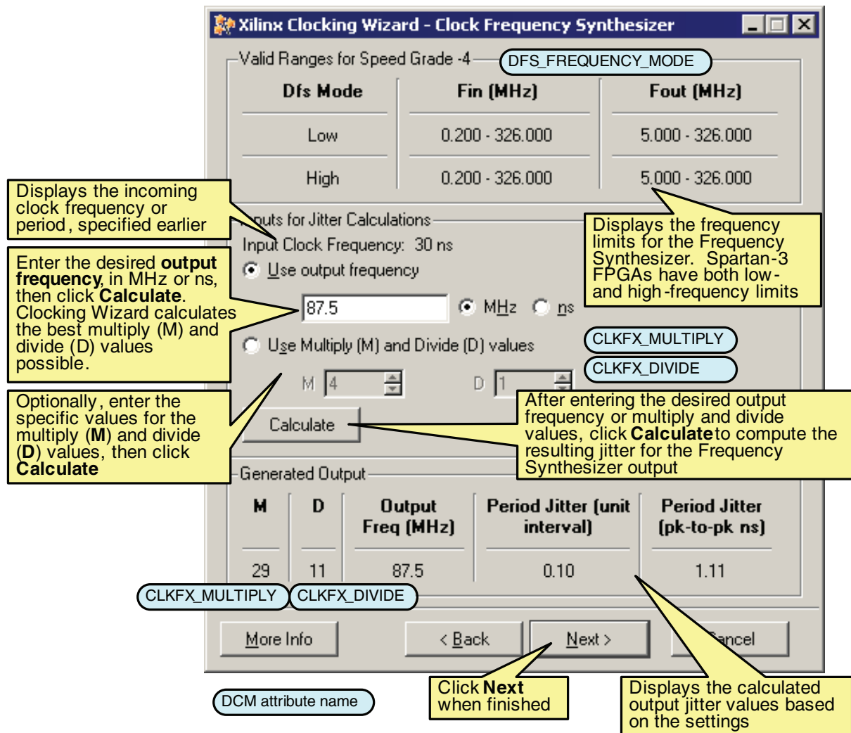
Figure 3-12: Set the Multiply and Divide Values for the Digital Frequency Synthesizer and Calculate the Resulting Jitter
