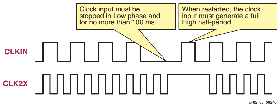
Figure 3-55: Momentarily Stopping CLKIN Clock Input
