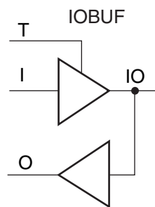
Figure 10-7: Input/Output Buffer (IOBUF) Symbol
