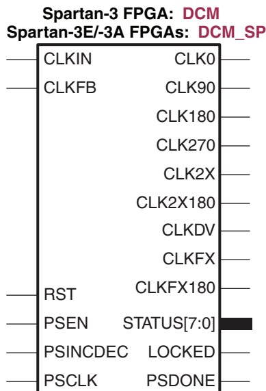
Figure 3-4: DCM Design Primitive
