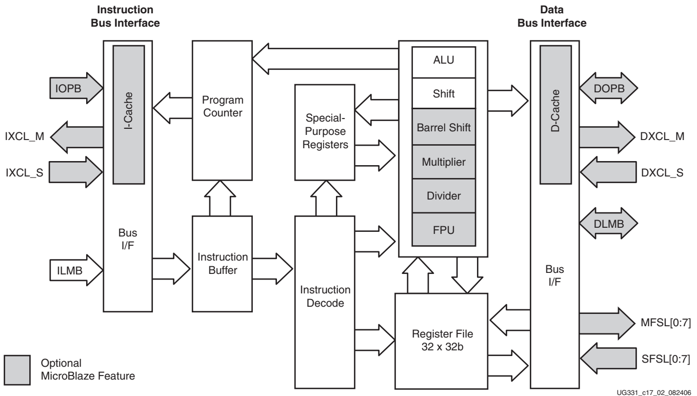
Figure 15-2: MicroBlaze Core Block Diagram
