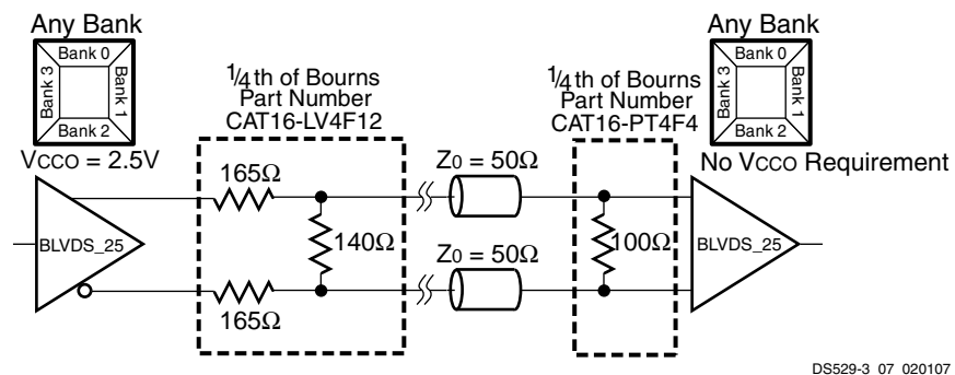
Figure 10-34: Spartan-3A/3AN/3A DSP External Termination Resistors for BLVDS I/Os
