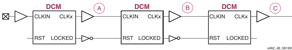
Figure 3-48: Calculating Jitter for Cascaded DCMs Depends on which DCM Outputs are Used
