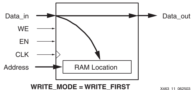
Figure 4-11: Data Flow during a WRITE_FIRST Write Operation
