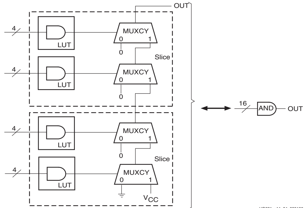
Figure 9-24: Library AND16 Implementation Using Carry Logic
