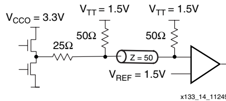
Figure 10-27: Terminated SSTL3 Class II
