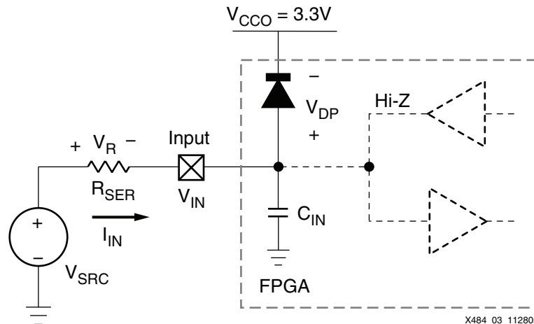
Figure 10-36: Series Resistor for V_{SRC} Greater than V_{CCO}+0.5V
