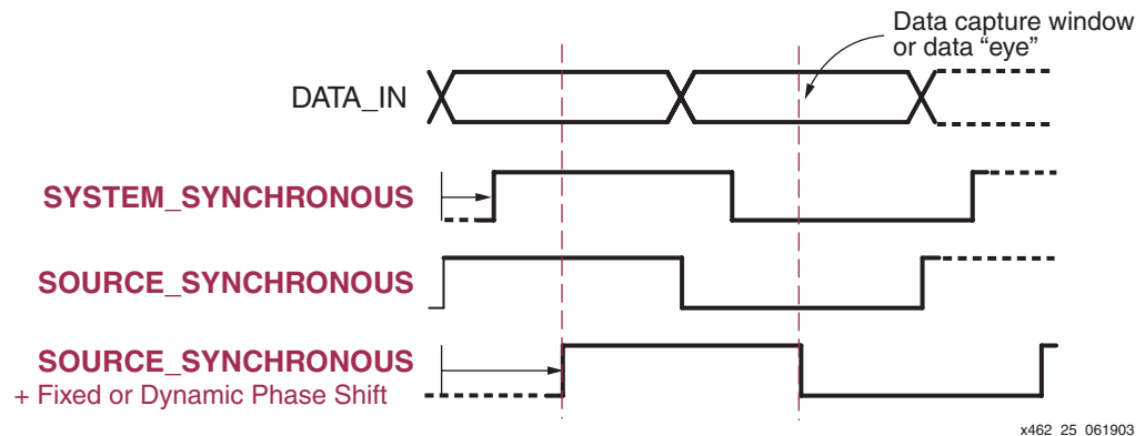
Figure 3-24: Comparing SYSTEM_SYNCHRONOUS and SOURCE_SYNCHRONOUS Timing in a Dual-Data Rate (DDR) Application
