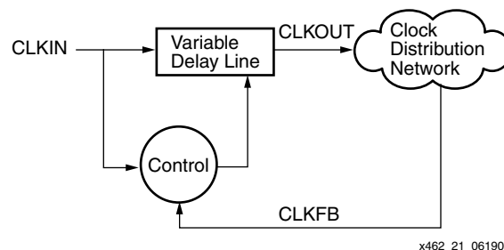
Figure 3-20: Delay-Locked Loop (DLL) Block Diagram
