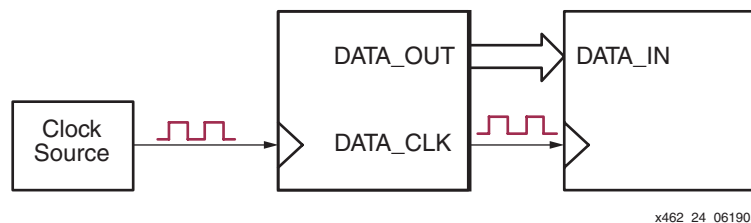
Figure 3-23: In Source-Synchronous Applications, the Data Clock is Provided by the Data Source
