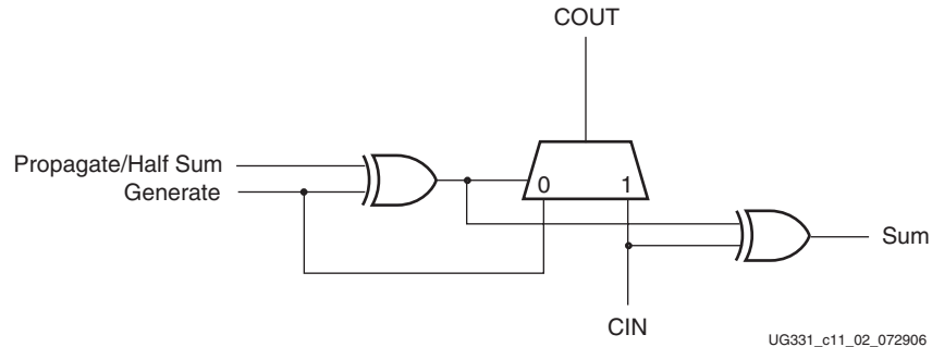
Figure 9-2: Look-Ahead Carry Implementation
