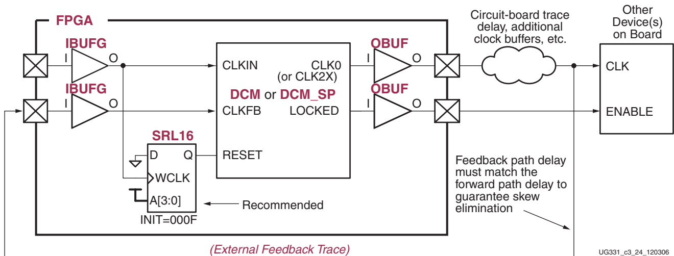
Figure 3-19: Eliminating Skew on External Clock Signals
