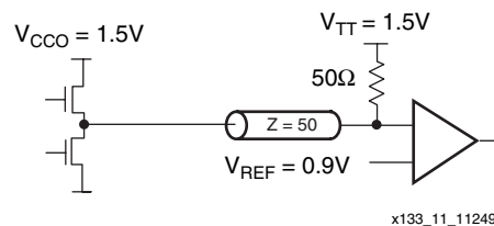
Figure 10-24: Terminated HSTL Class III
