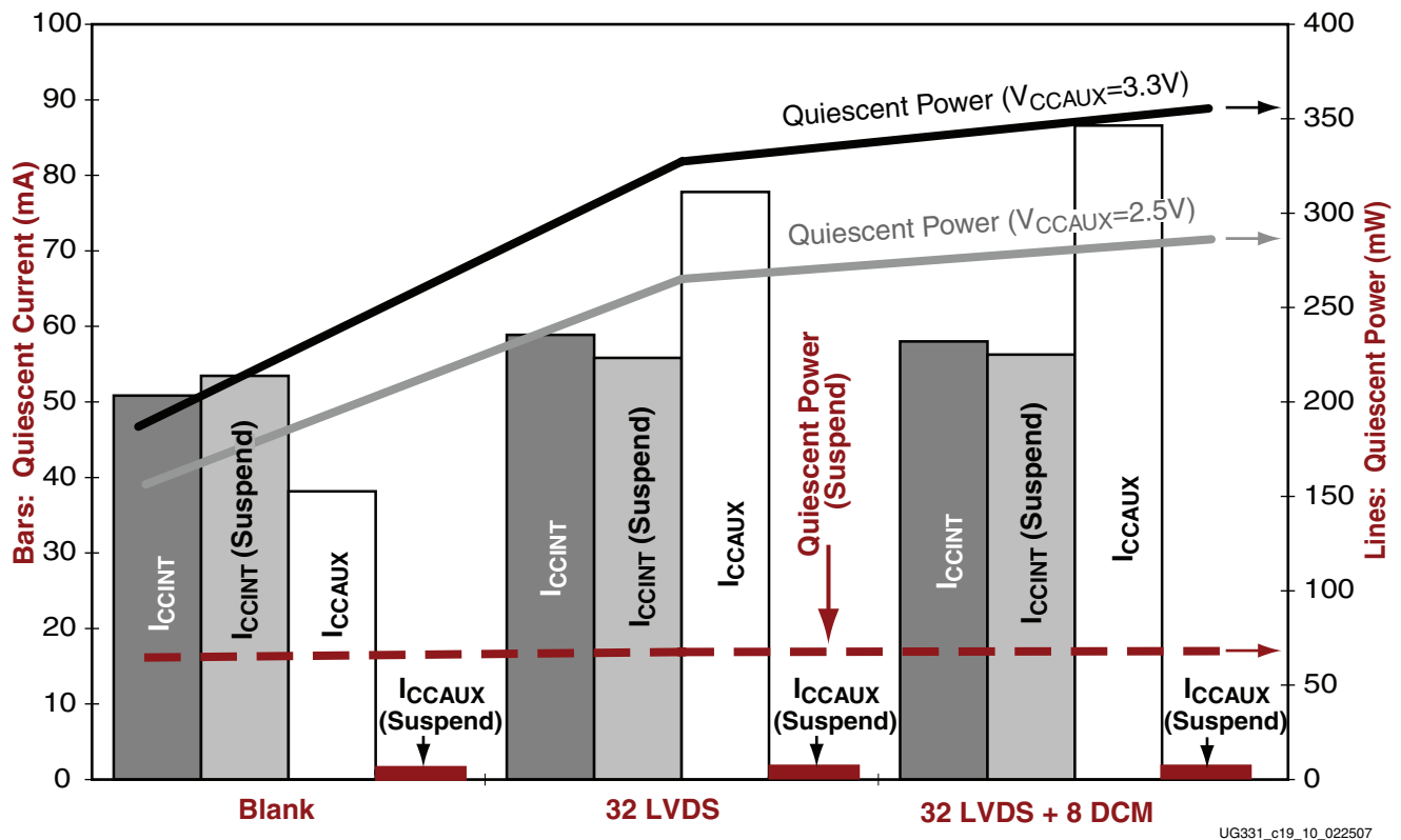
Figure 19-1: Effects of Spartan-3A Suspend Mode on Example Designs Measured on Typical XC3S1400A
