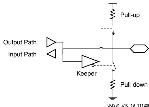
Figure 10-19: Keeper Circuit
