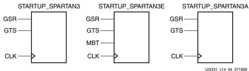
Figure 12-4: STARTUP Primitives for Spartan-3 Generation FPGAs
