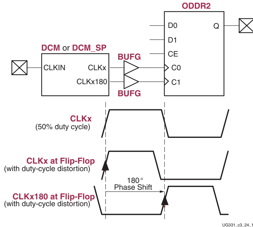
Figure 3-28: Using Half-Period Phase Shift Outputs Reduces Potential Duty-Cycle Distortion
