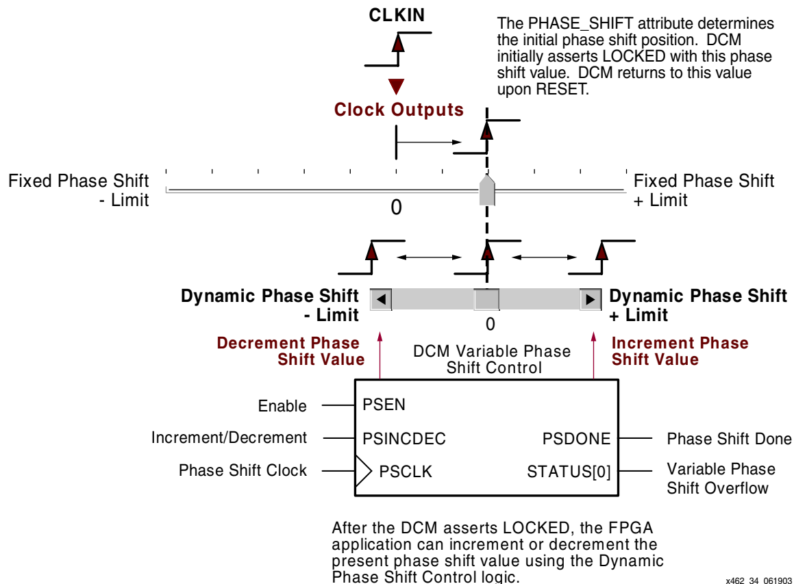
Figure 3-35: Variable Phase Shift Controls
